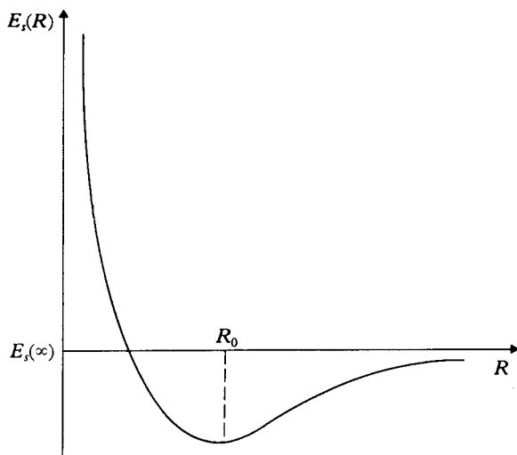
9.5 The general form of the electronic energy E_s(R) for a bound state of a diatomic molecule.
